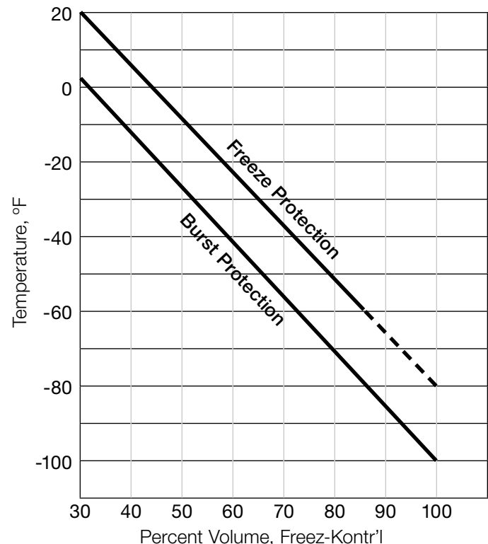
Figure 2 - Percent by volume required Freez-Kontr'l to achieve burst protection and freeze protection.
